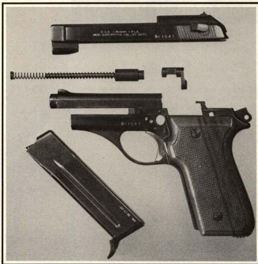
Super Titan II field-stripped
