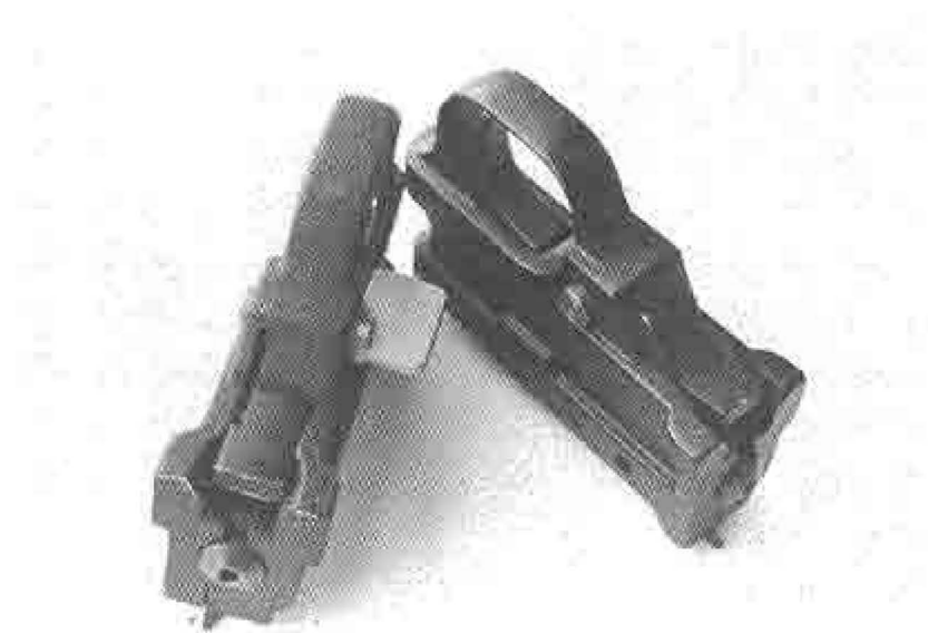
Bottom view showing the trigger housing assembly of the push-button-type safety of the factory (right) and the easily manipulated selector-lever-type of the converted model (left).
