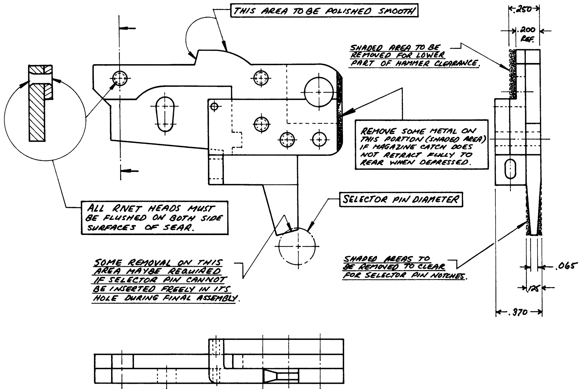
DETAIL-SEAR AFTER RIVETING AND FITTING
