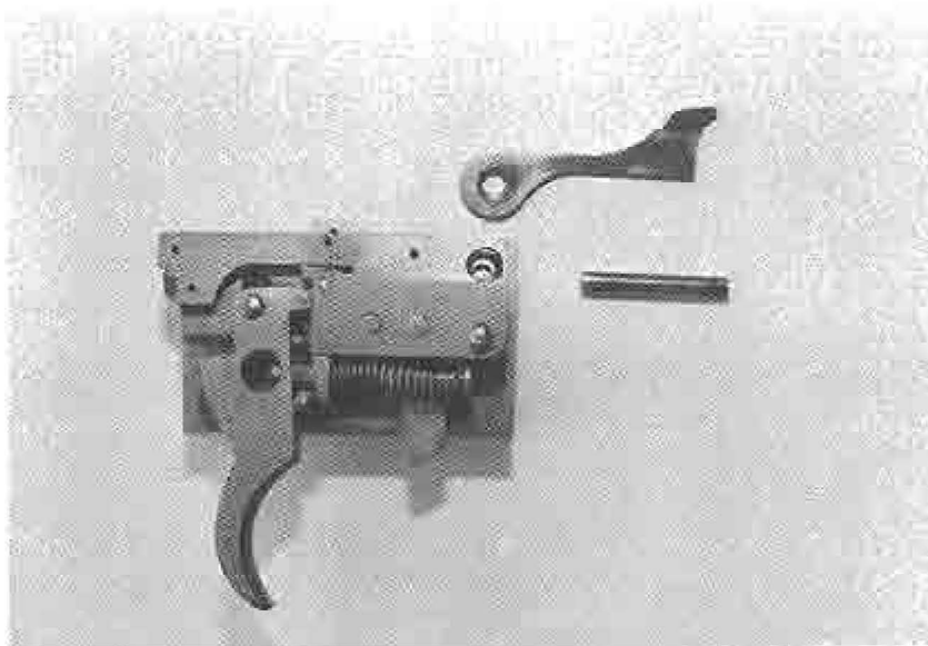
View of the conversion mechanism with the ejector disassembled. The ejector pin is assembled last and inserted in its usual hole.
