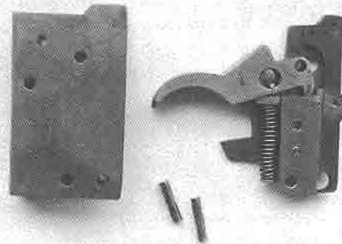
A view of the partially disassembled conversion unit. The two 1/8 -inch diameter pins securing it to its housing were removed. These two pins act as pivot pins for the sear and trigger.
