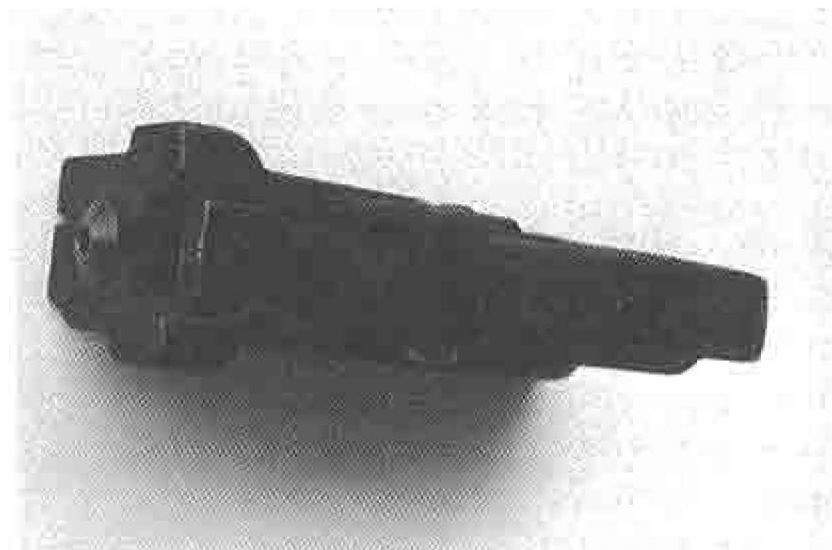
Photo shows the slave pin assembled in the selector pin hole. This pin must be in place prior to assembling the weapon to the stock. After the gun has been assembled to the stock, and the stock screw has been tightened, the slave pin is pushed out by the selector lever pin.
