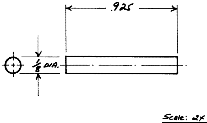
HAMMER PIN
