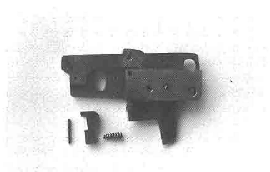
Sear group is shown disassembled. The trip and its spring are removed from the sear. Here a small internal spring is improvised from watchband plunger spring and inserted into the normal spring for additional power.
