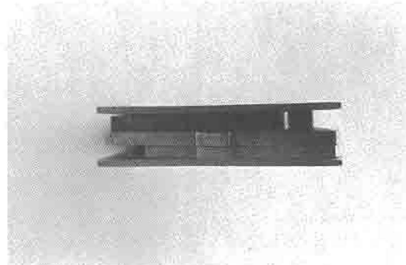
Top view of the fully assembled conversion unit. Note the clearance gap on the right side of the sear for hammer travel during operation.
