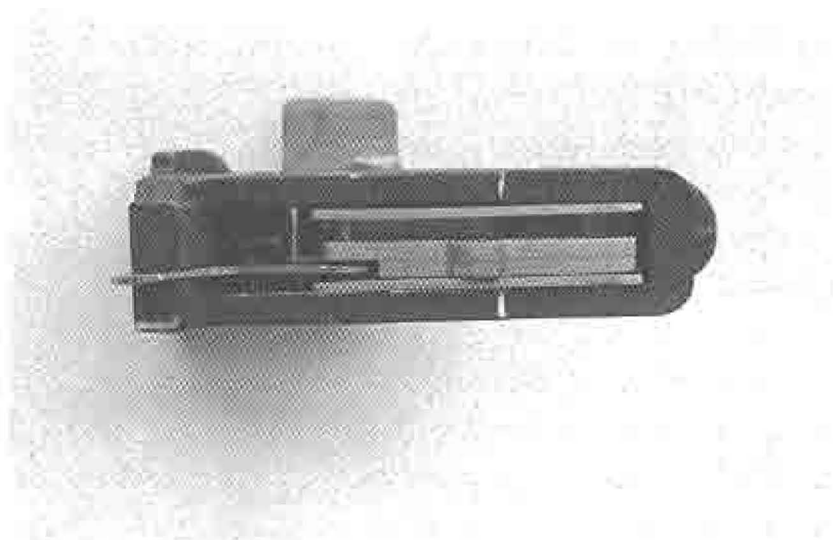
Top view showing the converter mechanism assembled inside the factory trigger housing frame. Note the sear clearance for the ejector. Note also the gap on the right side of the sear where the lower part of the hammer will travel during operation.
