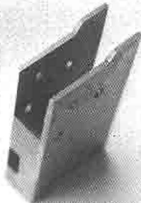
Detailed rear top view showing the conversion unit housing improvised from a rectangular piece of tubing with external measurements of 1/2 \times 2 inches of 1/16 -inch sheet metal. This material is commonly used by furniture manufacturers.
