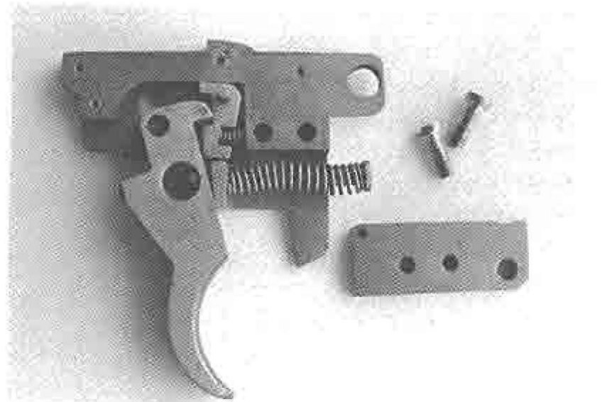
View of the sear/trigger assembly with the spring rod and spring in place.
