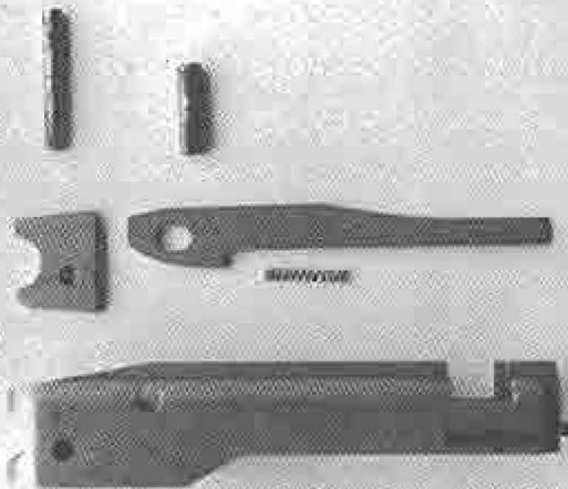
Bolt assembly but with the firing pin adapter substituted for the original factory trigger mechanism.
