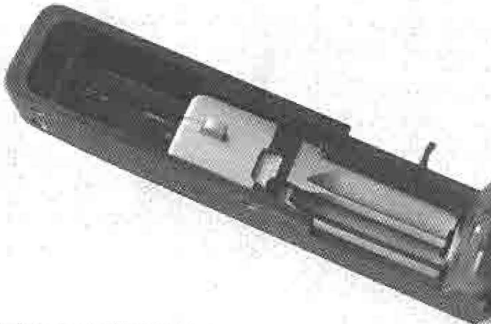
View showing the bolt mechanism fully assembled inside the receiver housing. In this view, the pivoting hammer design used for selective-fire is installed, and the hammer's lower part protrudes underneath the bolt rear end. The lower protrusion of the hammer in the underside of the bolt will hit the ignition shoulder (ejector pin) during bolt closure to fire the weapon.
