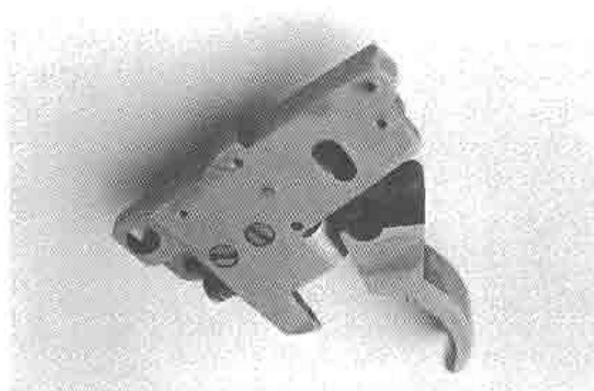
Top rear view showing the conversion trigger mechanism fully assembled. Note the step on the top left side of the trigger where the left piece of the sear is resting. This step allows clearance for sear action. The oblong slot on the rear portion of the sear allows clearance for the trigger pin and sear motion.
