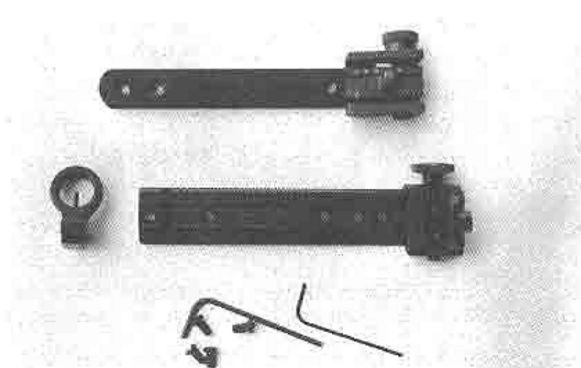
Photo showing the ultimate "military sighting system" for use on the 1022. At top is the M1 30 carbine military adjustable system mounted on a dovetail slot on top of the factory supplied scope base. Below is Feather Enterprise's innovative adjustable rear sight that is easily installed via the scope base supplied with the sight. Both the rear sights pictured will perfectly match the H&K front sight.
